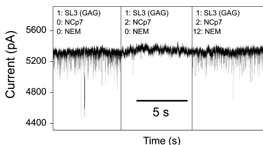
Figure 6. Effect of N -ethylmaleimide on formation of the NCp7–SL3 RNA complex. Event frequency modulation caused by the addition of 5 \mu\text{M} high-affinity SL3 (GAG) aptamer, with 10 \mu\text{M} NCp7, causing reduction in the event frequency. Introduction of 60 \mu\text{M} N -ethylmaleimide returns the event frequency to near its pre-NCp7 level. The applied transmembrane potential was +400 mV. The buffer solution contained 200 mM NaCl, 5 mM \text{NaH}_2\text{PO}_4 , pH 7.0 on the cis side and 1 M NaCl, 5 mM \text{NaH}_2\text{PO}_4 , pH 7.0 on the trans side. The nanopore was \sim 6 nm in diameter in a 15 nm thick nitride.
